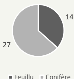
Volume (Mm 3 )
