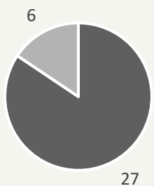
Volume (Mm 3 )
